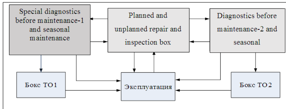
Fig. 1. An approximate diagram of relations of various equipment and elements for the analysis of the SPRS reliability.
