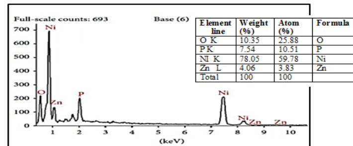
Fig11. EDAX spectrum showing presence of Ni-P coated on magnesium (Mg) composite reinforced with multiwall carbon nanotube (MWCNT) at varying % of ZnO (a) 0.1% (b) 0.5% (c) 1% (d) 2%, with surfactant (SLS).
