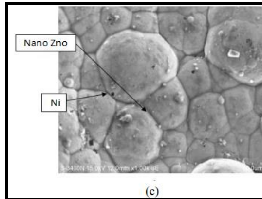
Fig10. SEM micrograph (1000X) of electroless Ni-P coating on magnesium (Mg) composite reinforced with multiwall carbon nanotube (MWCNT) at varying % of ZnO (a) 0.1% (b) 0.5% (c) 1% (d) 2%, with surfactant (SLS).
