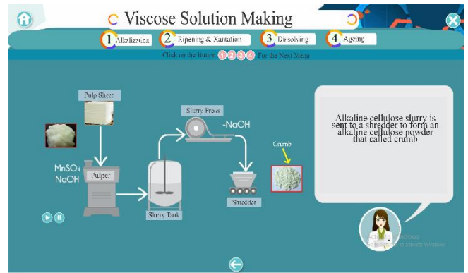
Figure 4. One of the Virtual Textile Chemistry Laboratory Content (The making of Liquid mixture of Viscose on Alkalinity Process)
