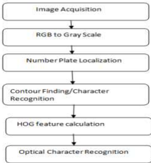
Fig: Block Diagram for the Proposed Algorithm
